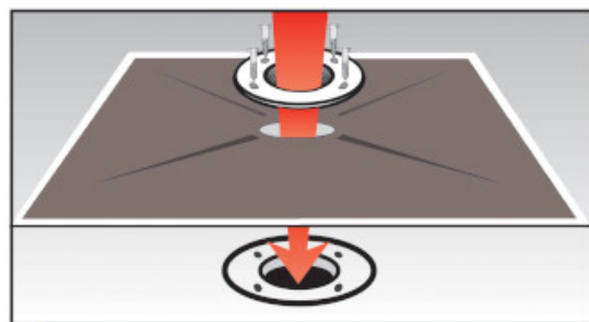
Square rubber element for flexible waterproofing and sealing of a 425 mm x 425 mm drain
